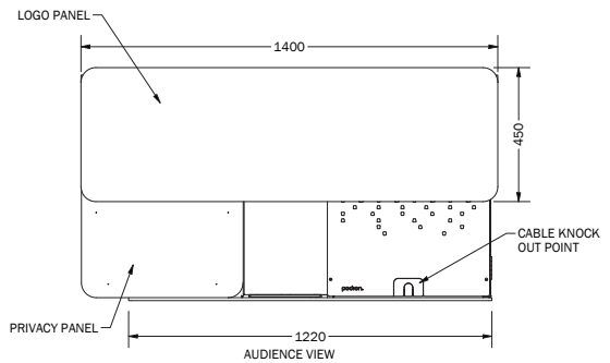
AUDIENCE VIEW
