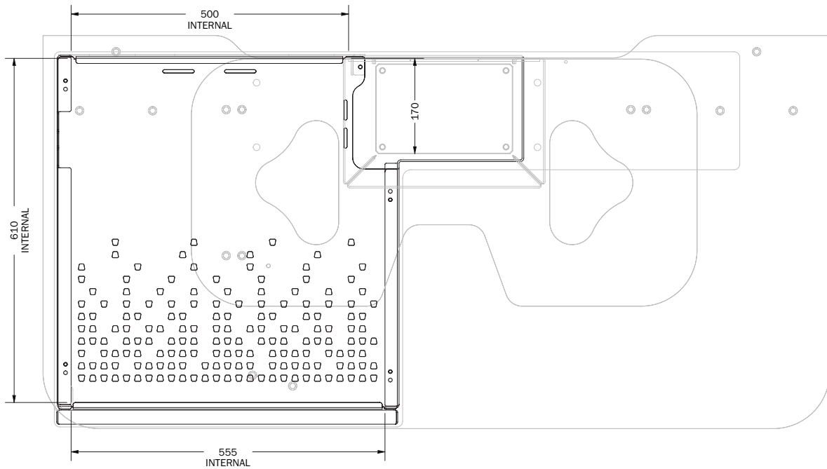
TDP-EV-L ORIENTATION SHOWN
