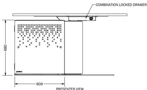
PRESENTER VIEW
