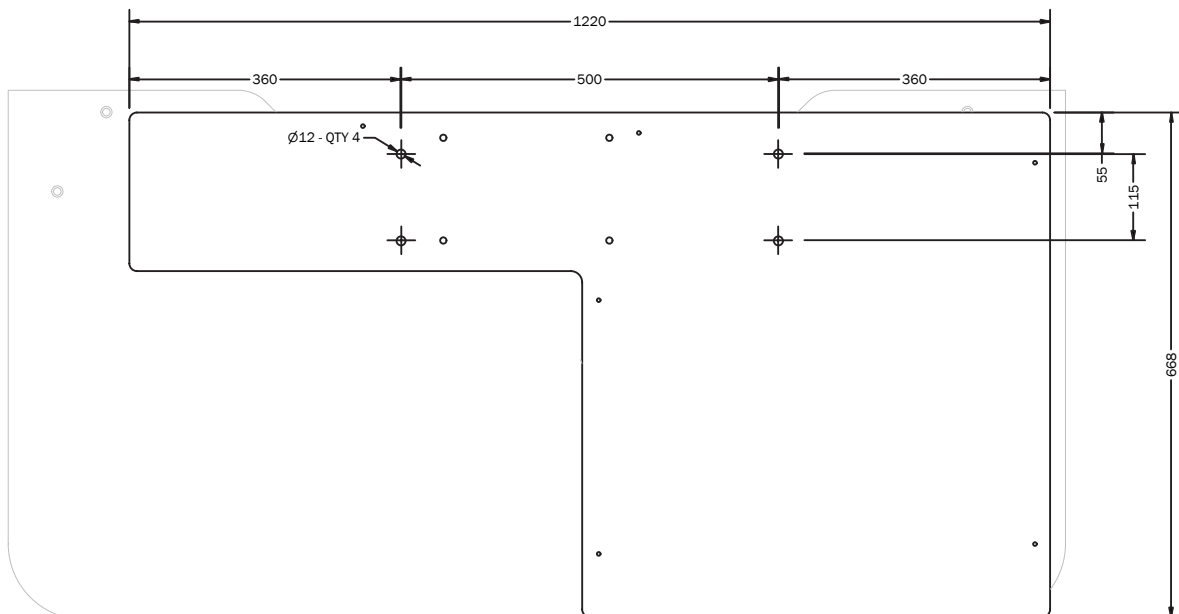
BOTTOM VIEW
