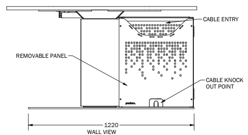
WALL VIEW
